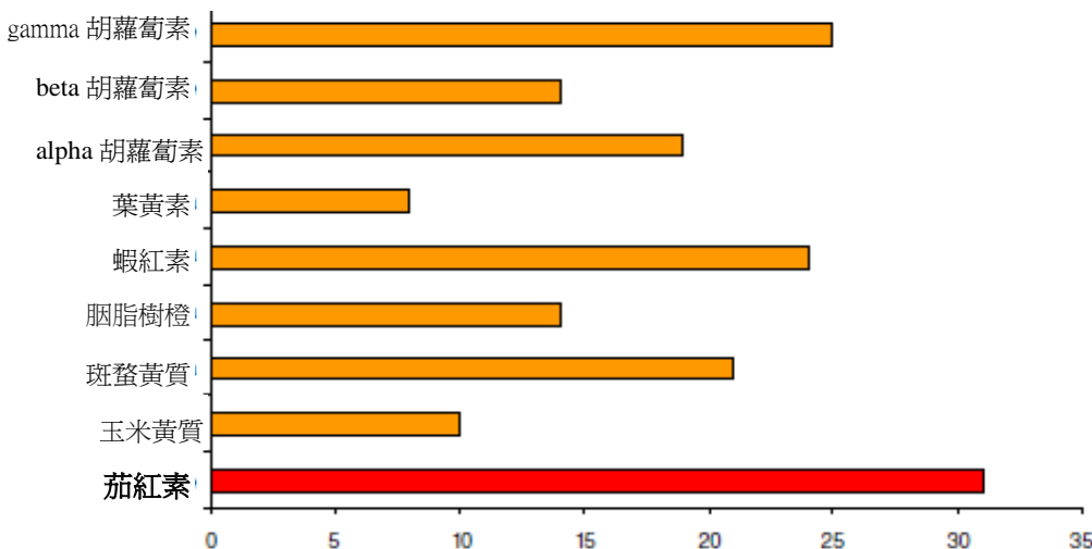
Figure 2: Quenching constant values against singlet oxygen of some carotenoids.
